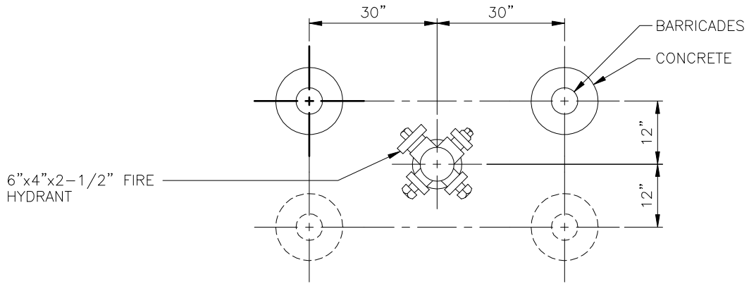
TYPICAL FIRE HYDRANT BARRICADES FOR STREETS WITHOUT CURBS
