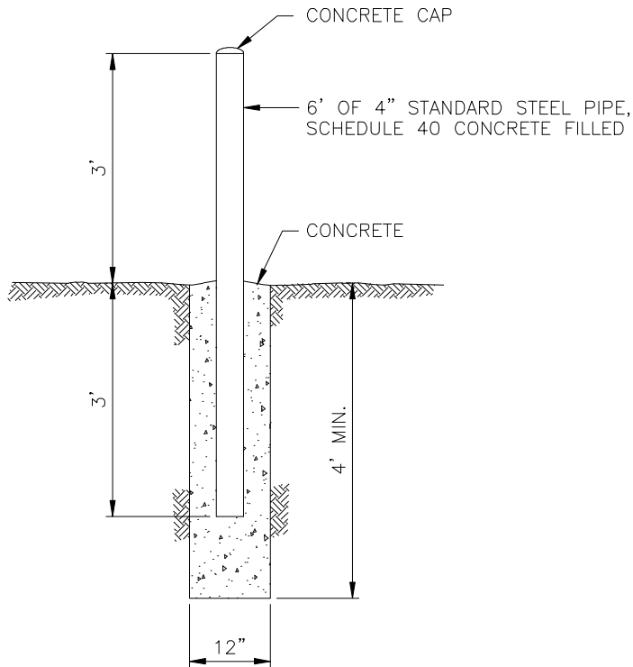
BARRICADE DETAILS
